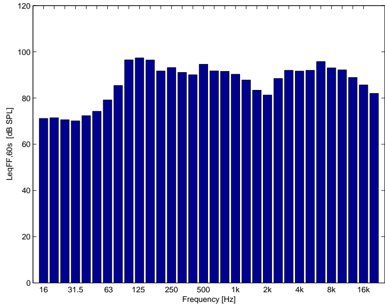
Figure C.3: L_{eqFF,60s} in third octave bands calculated after the free field correction. The data after the free field correction is shown in Figure C.2. The data show in this graph is an average of the right and left ear.
