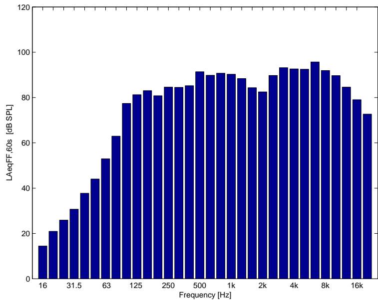
Figure C.4: L_{AeqFF,60s} in third octave bands calculated after the free field correction and the A-weighted correction. The data after the A-weighted correction is shown in Figure C.3. The data show in this graph is an average of the right and left ear.
