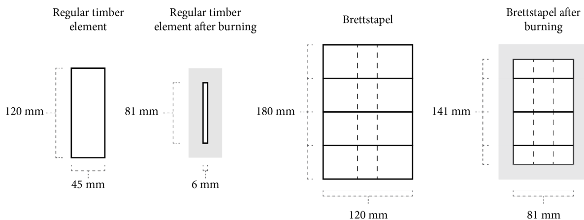
Figure 62: Comparison of a mink farm timber element and four of the same element assembled by dowels, after 30 minutes of burning.
