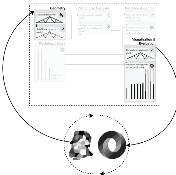
Figure 46: Wallacei iteratively changes the geometry in order to approximate the best performing structure, this data is saved by JSON, allowing each iteration to be recorded and reinstated.
