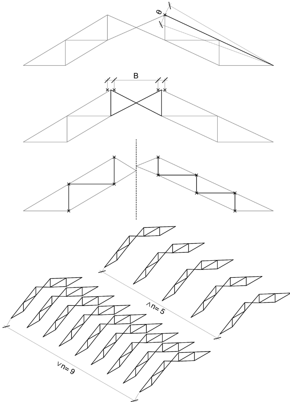
Figure 64: Variables which can be influenced by Wallacei for the search of an optimized solutions. These include the roof shape, width of roof ridge, amount of web elements and amount of total trusses.
