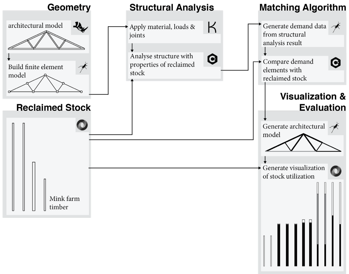
Figure 41: Overview of the tool, illustrating the role of each component and their associated software.
