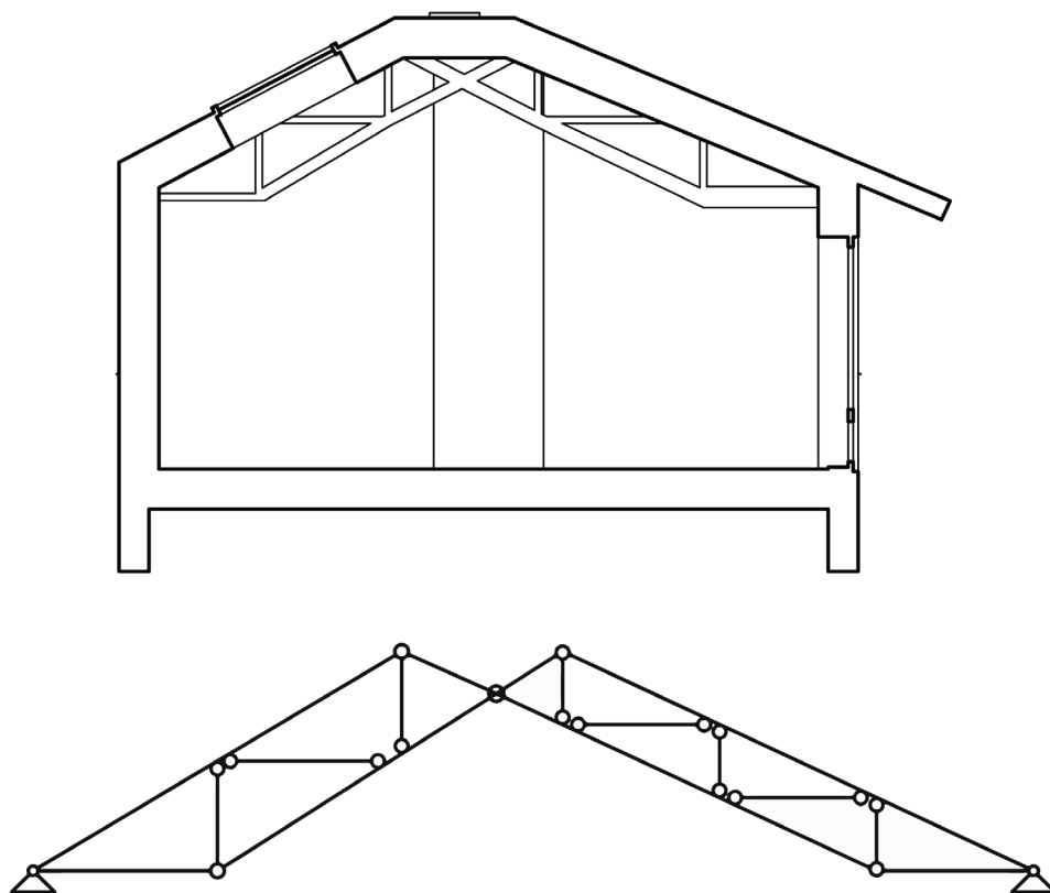
Figure 61: The selected truss and a freebody-diagram representing the joints and supports of the structure.
