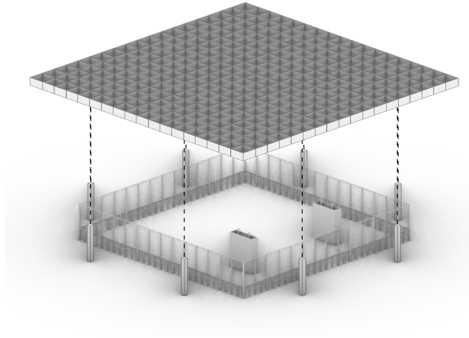
Figure 84: Exploded axonometric of the structure in Neue Nationalgalerie.
