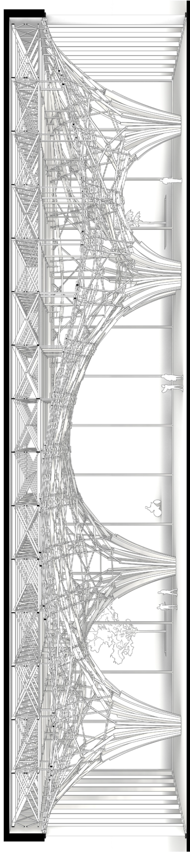
Figure 91: Section of structure #1 in 1:200.
