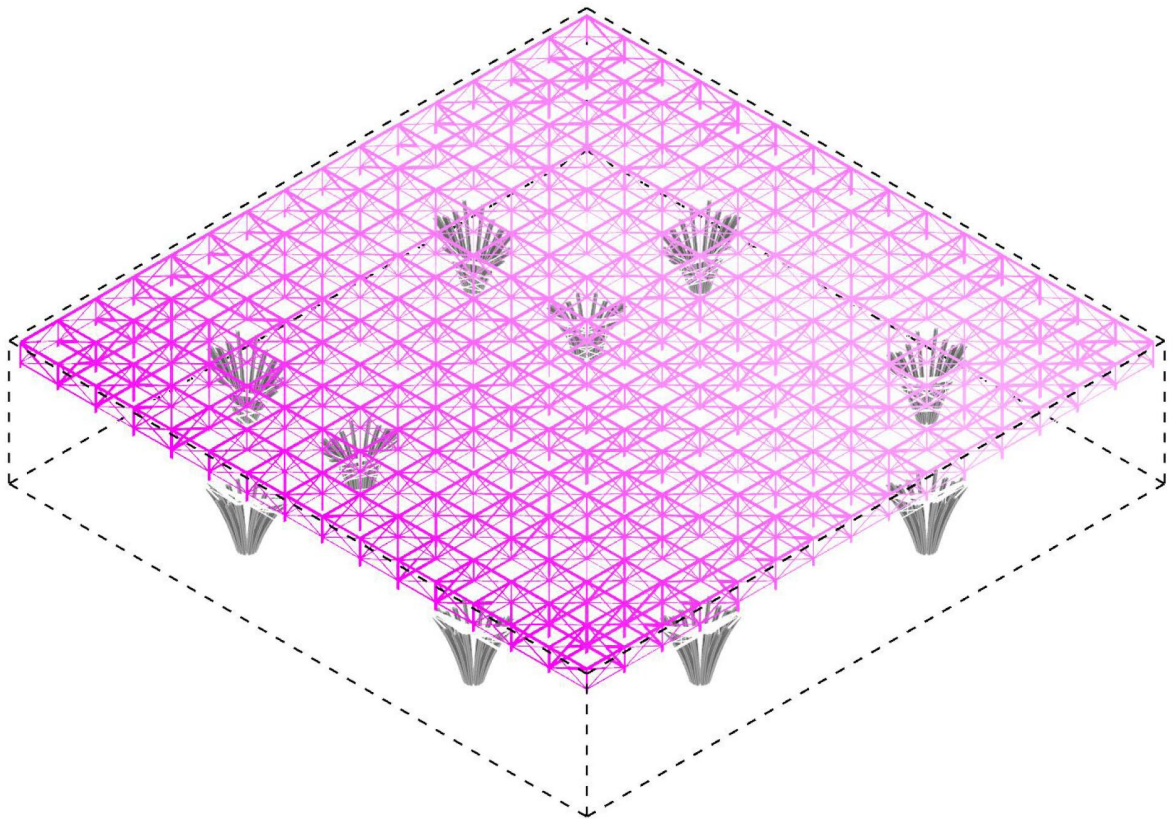
Figure 87: Diagram showing the deformation of a structural analysis performed of the space frame.
