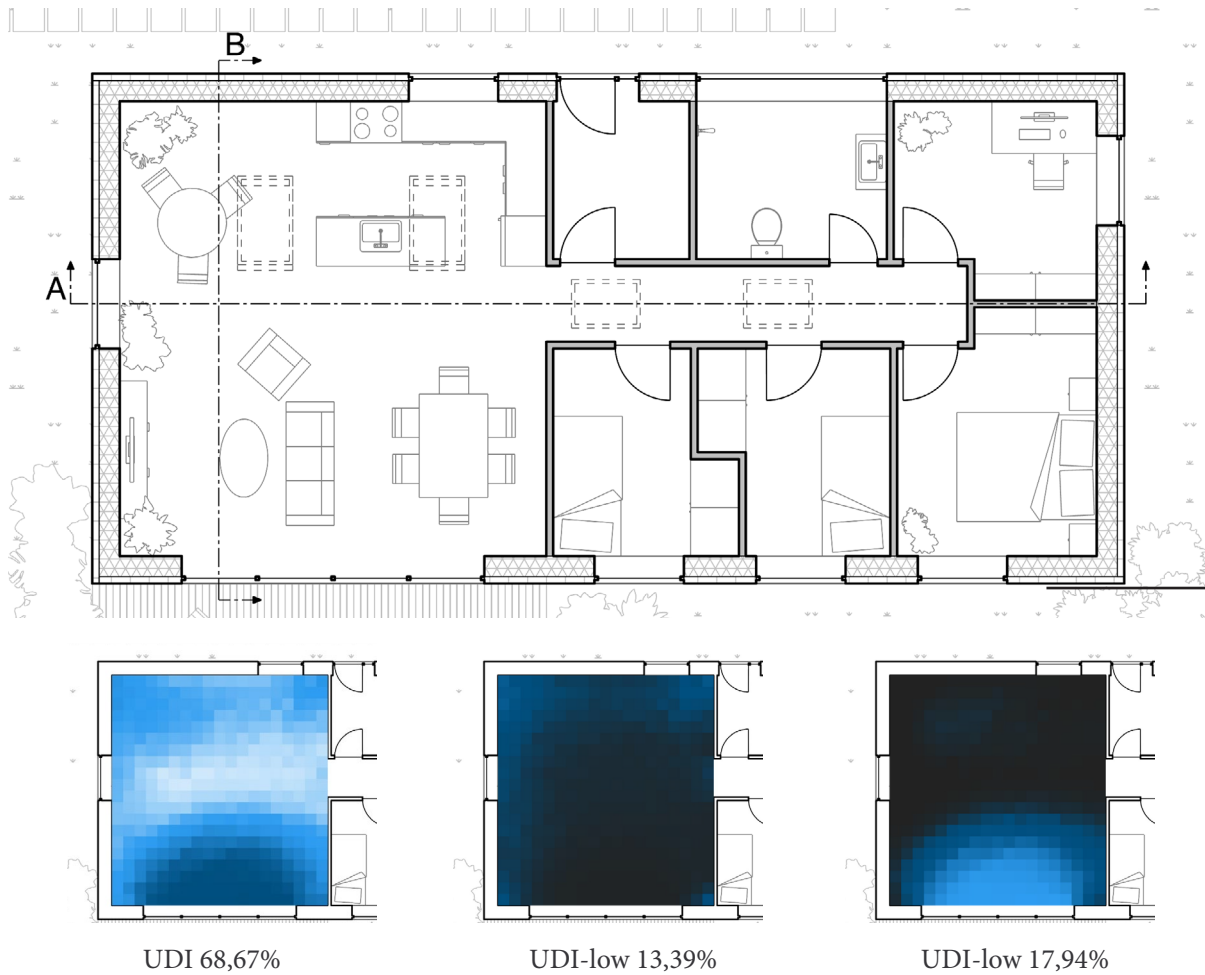
Figure 72: Plan in 1:100 after renovation along with the daylight results, seen below the plan.
