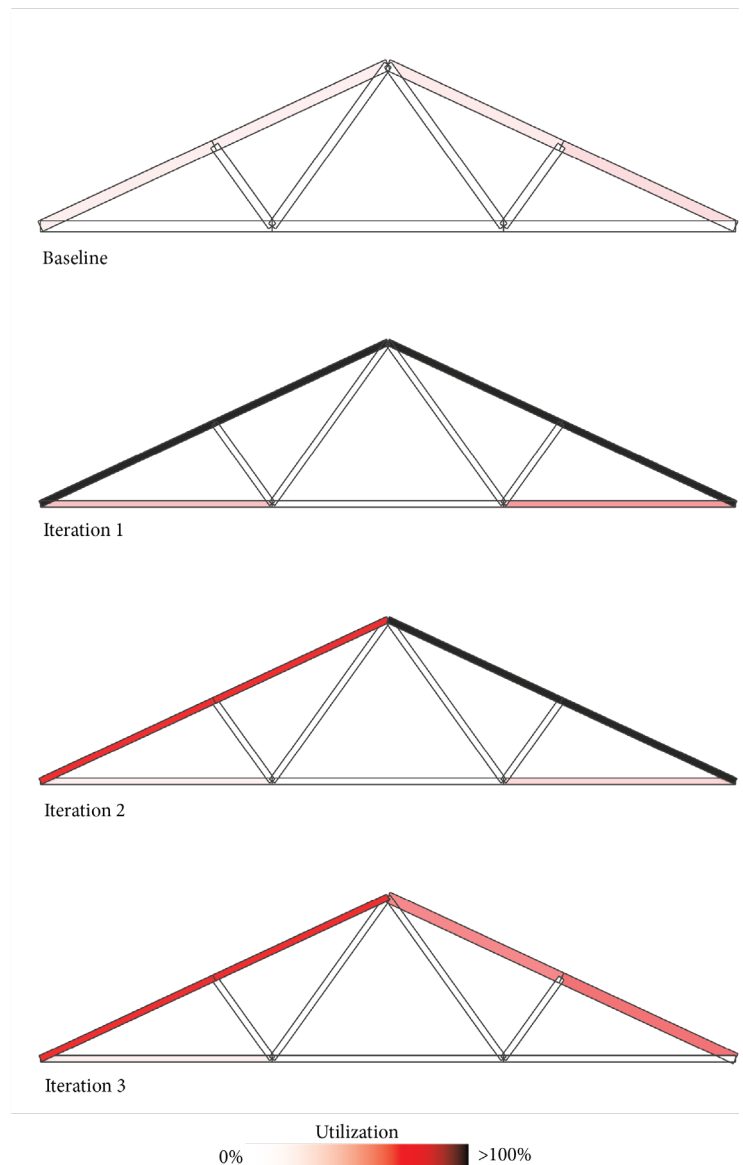
Figure 43: The cross section optimization algorithm iteratively replaces structurally overutilized elements with a stronger cross section. The structural analysis needs to be iterative, as the forces transfer in different ways each time a cross section is replaced. The algorithm is done once every element is below 100% utilization, in this case needing three iterations.
