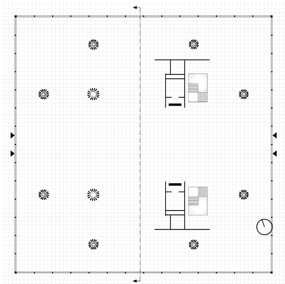
Figure 89: Plan of structure #1 in 1:300.
