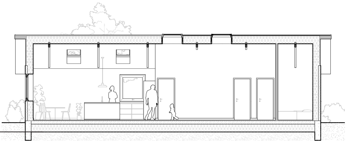
Figure 73: Longitudinal section A in 1:100.
