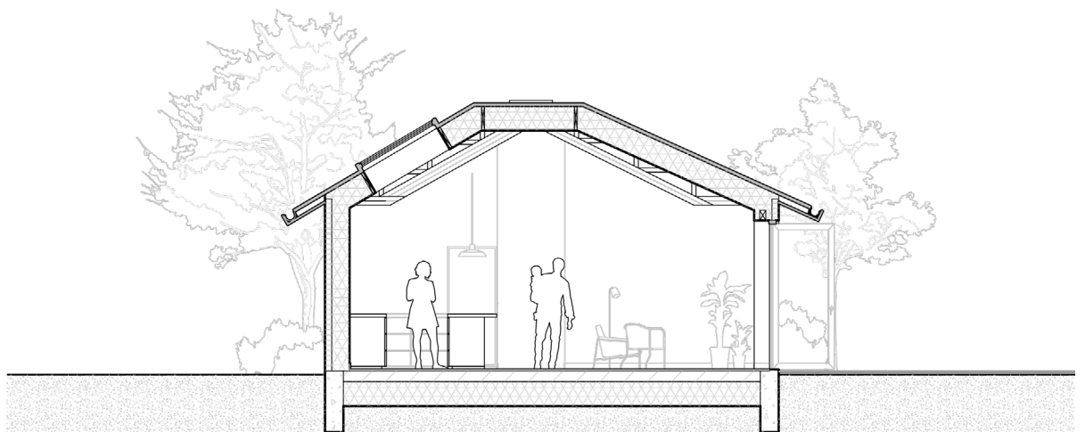
Figure 74: Lateral section B in 1:100.
