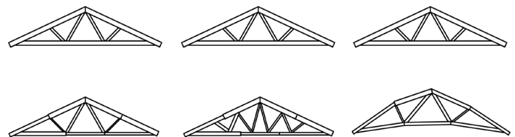
Figure 31: Diagram of the baseline, moderate and advanced levels of optimization, gradually increasing the impact on the design.
