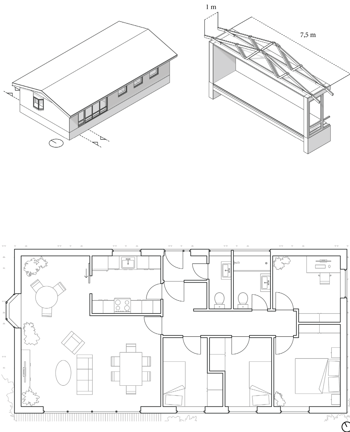
Figure 53: The residential house as it stands before renovation. Axonometric (above) of the exterior and existing structure. Plan (below) in 1:100.
