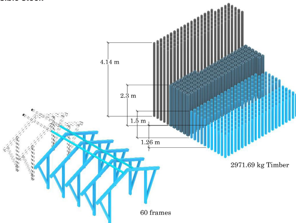
Figure 52: Accessible stock for Design Study #1 equivalent to a single wing.
