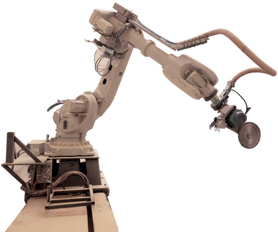
Figure 23: Picture of an ABB robot used at Woodstock Robotics. Author's own photograph.
