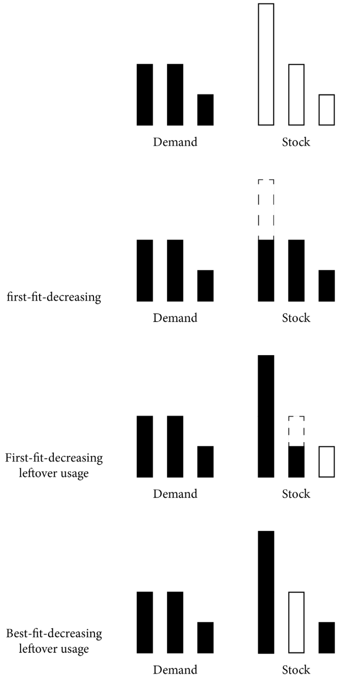
Figure 35: Algorithms for solving the cutting-stock problem in relation to the problem of the thesis.
