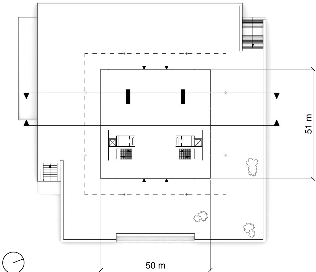
Figure 82: Plan of the existing plan 1:500
