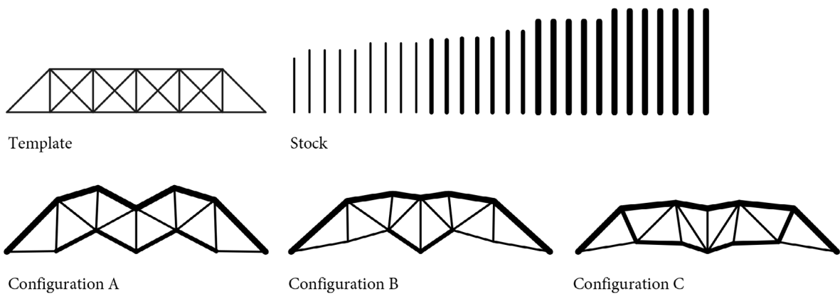
Figure 15: Diagram of the first approach, stock-constrained structural analysis. Adapted from Brütting et al. (2019).
