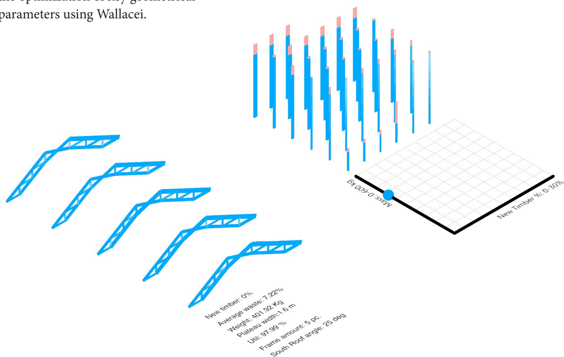
Figure 77: Diagram of the structure, stock usage and associated data.
