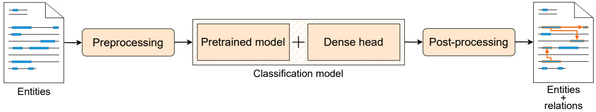
Figure 6: RE system overview.
