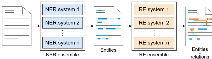
Figure 4: Information extraction pipeline overview.
