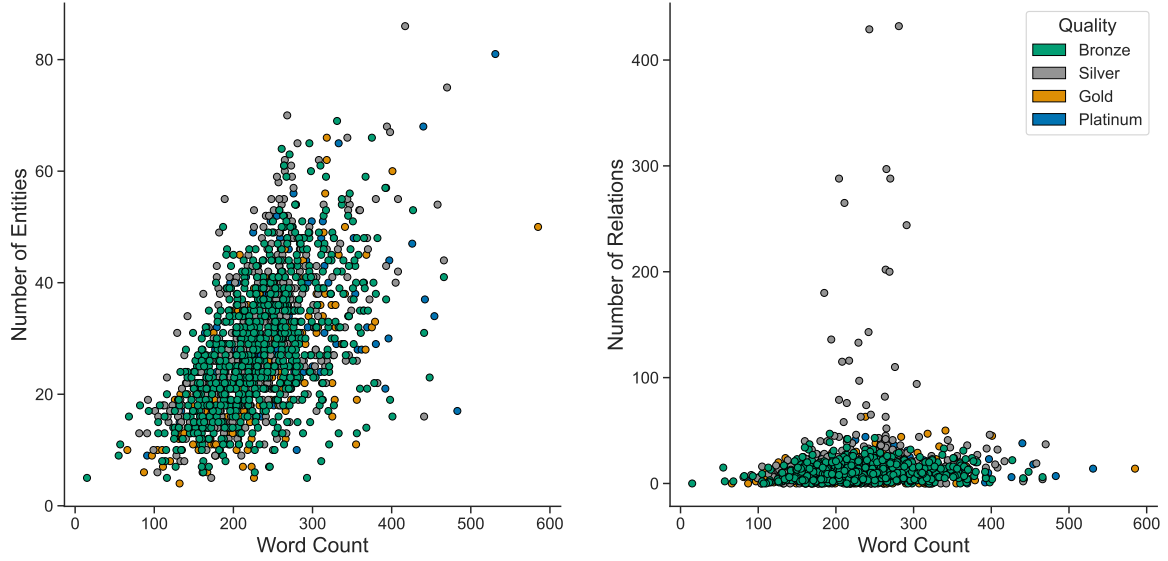
(a) Number of entities vs. word count for all articles. (b) Number of relations vs. word count for all articles.
