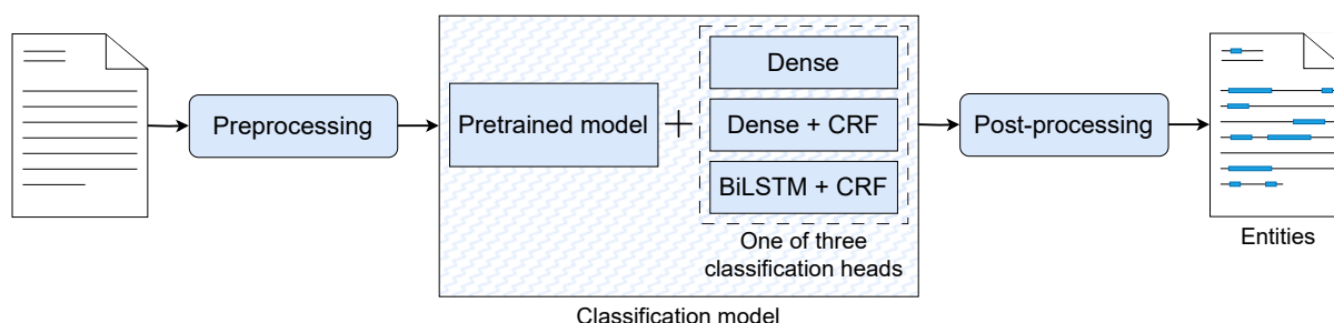
Figure 5: NER system overview.
