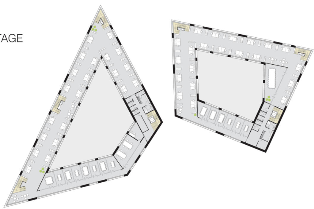
FJERDEETAGE 1:750
